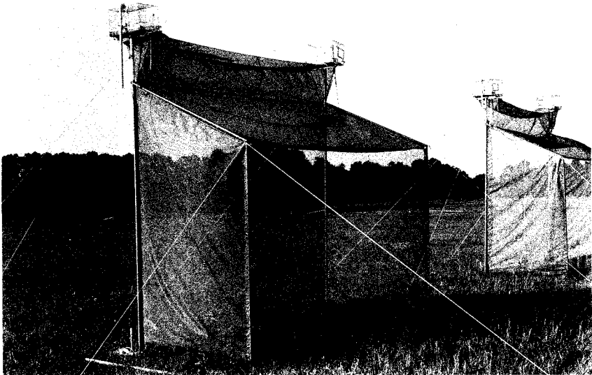
FIG. 1. Standard traps. Trap in foreground is of polyester mosquito netting; the other has the main wall and back of duct of monofilament shrimp net.
