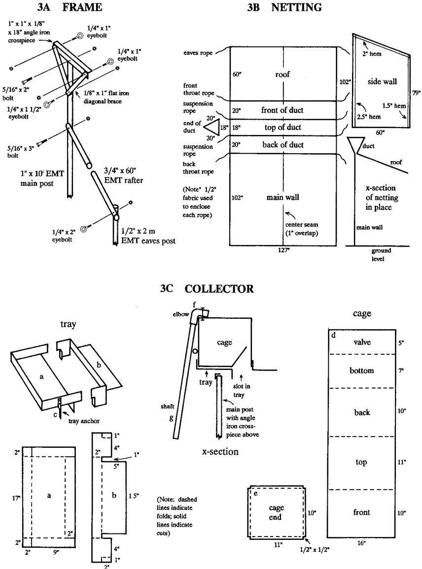
FIG. 3. Construction details of standard trap. (Dimensions are in inches: 1" = 2.54 cm.)
